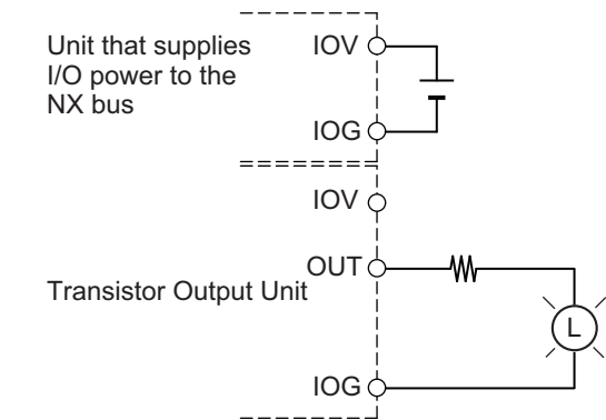
PNP type
