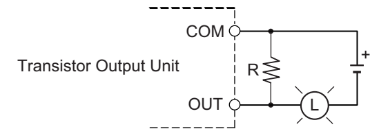
PNP type
