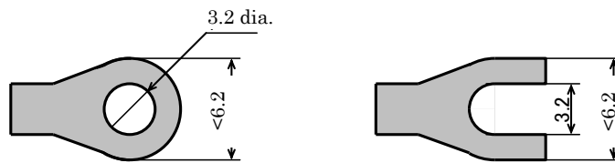
Recommended Crimping Terminal
