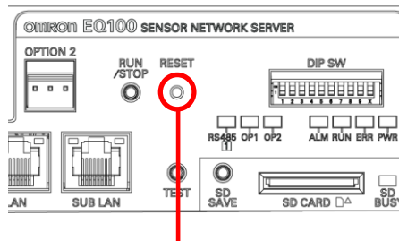
RESET Button
