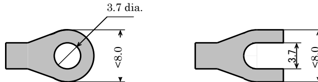
Recommended Crimping Terminal
