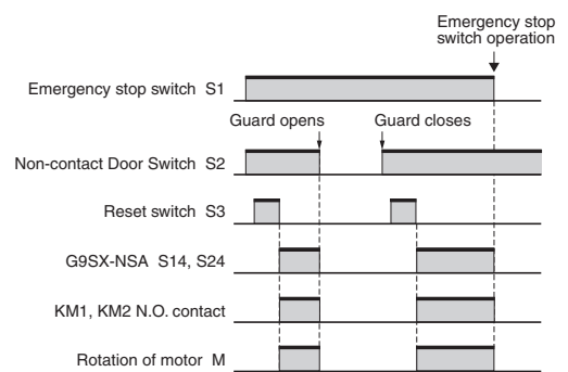
Timing chart
