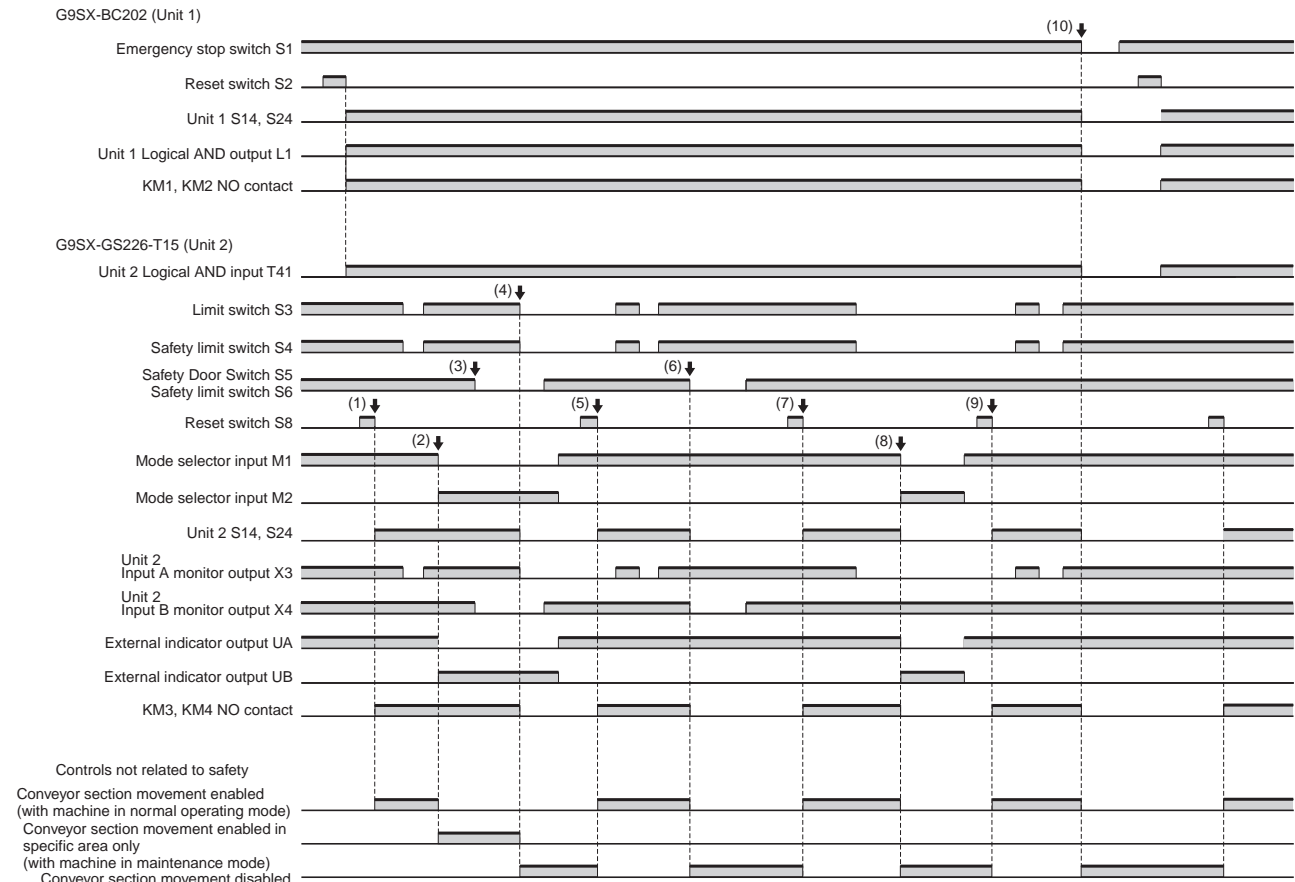
Timing Chart 2
